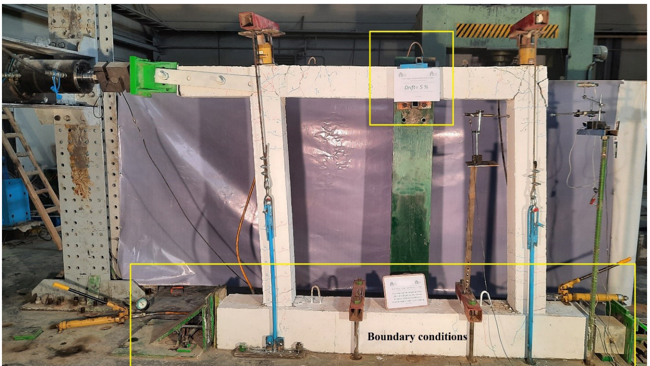
Fig. 5 Properties of the experimental specimen with lateral restraining of the frame
