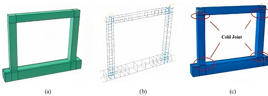
Fig. 10 Numerical model; (a) Geometry of the concrete section in the monolithic concrete model; (b) Geometry of rebars and stirrups; (c) Geometry of the CJ model
