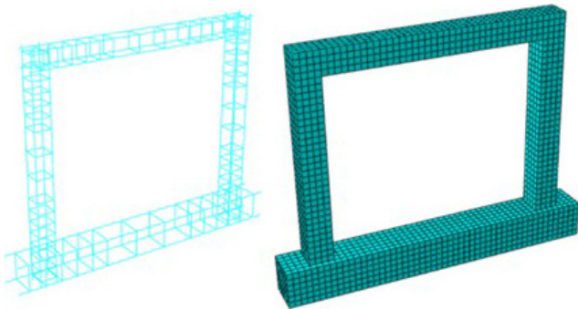
Fig. 12 Meshing the concrete part and reinforcement
