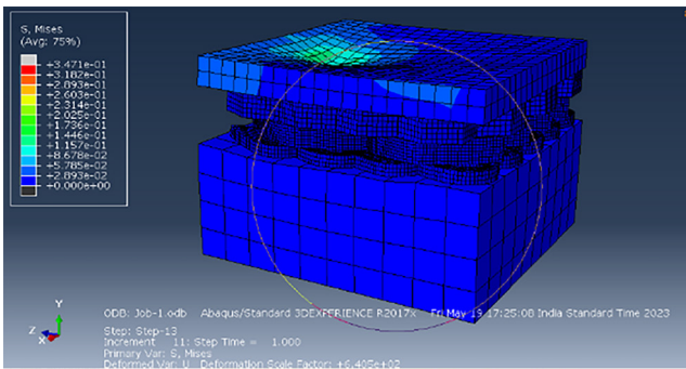
Fig. 8 Simulated view of novel flexible pavement design
