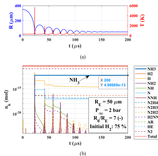
Fig. 1 A typical example of the dynamics of a freely oscillating microbubble: (a) bubble radius and internal temperature as a function of time, (b) temporal evolution of the chemical species in moles
