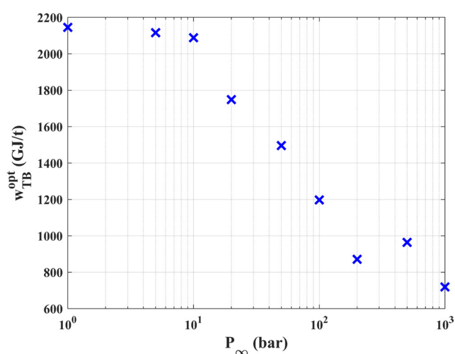
Fig. 5 The optimal energy intensity of the ammonia production versus the ambient pressure
