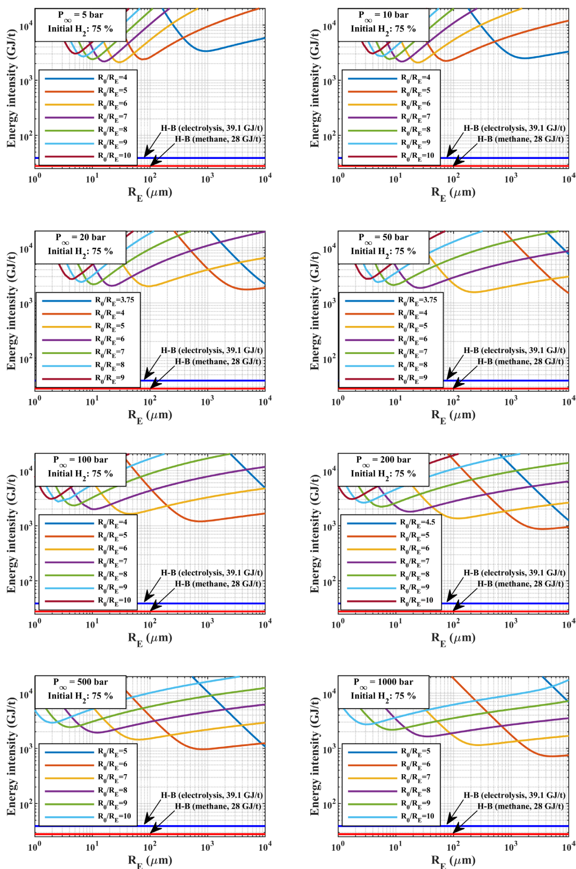
Fig. 4 The energy intensity of the ammonia production at several ambient pressures
