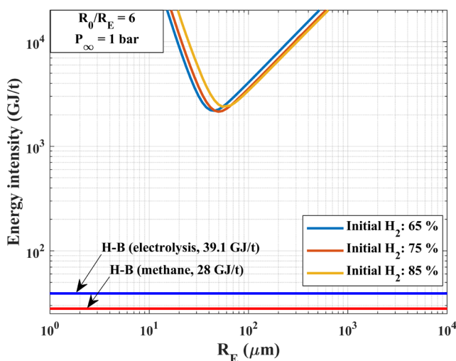
Fig. 3 The effect of the mole fraction of hydrogen on the energy intensity of the ammonia production at the best relative expansion from Fig. 2
